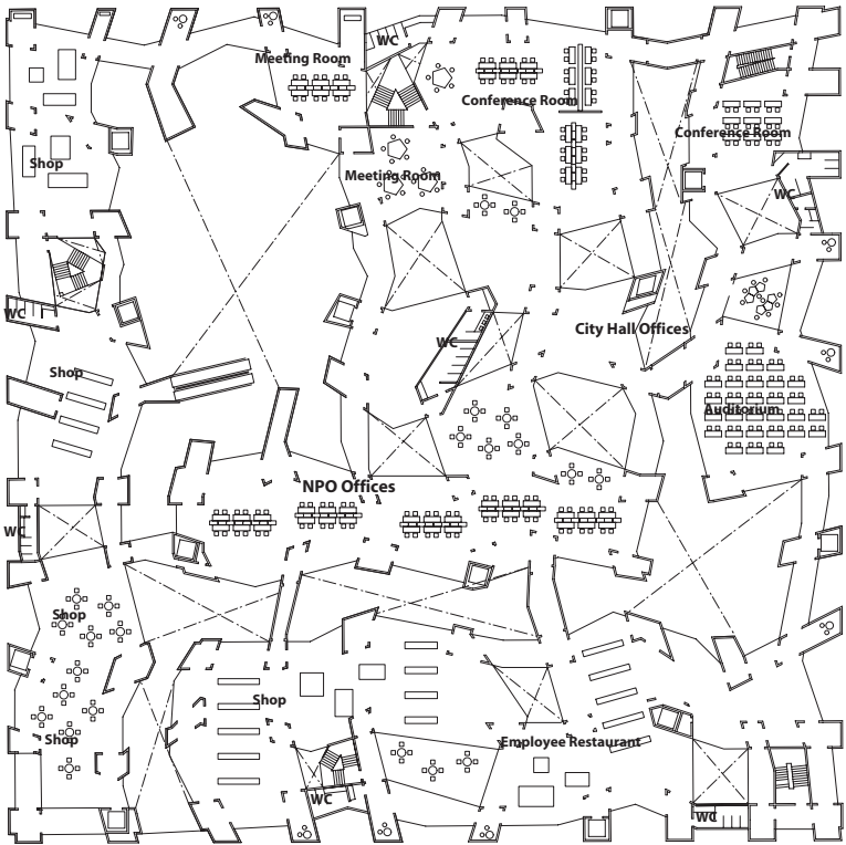
3F-6F (Office Floor) Plan 1/500
