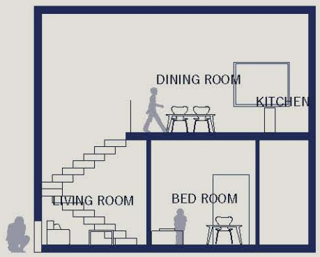
SECTIONPLAN
