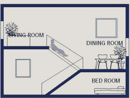
SECTIONPLAN
