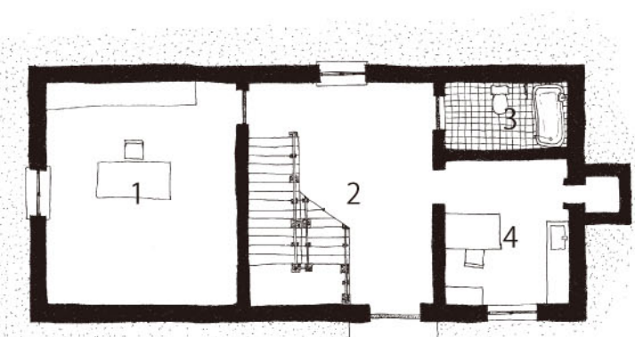
Ground floor plan S=1:200
