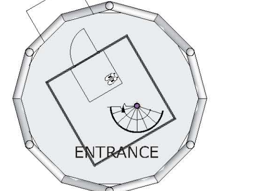
First floor;scale:1/100
