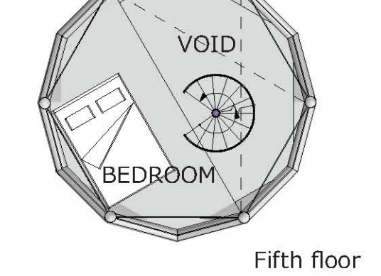
Fifth floor
