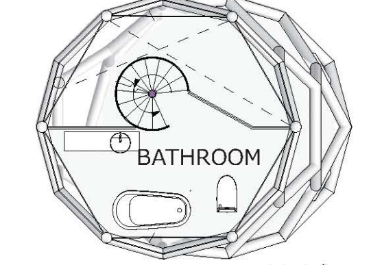
Third floor
