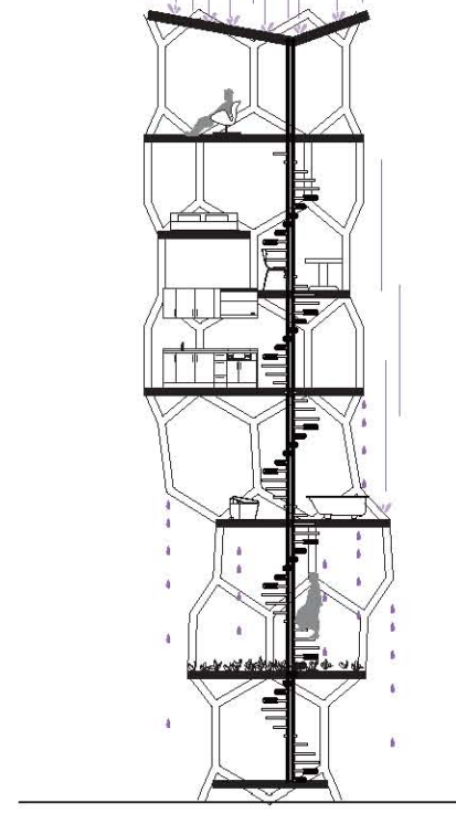
section;scale:1/200
