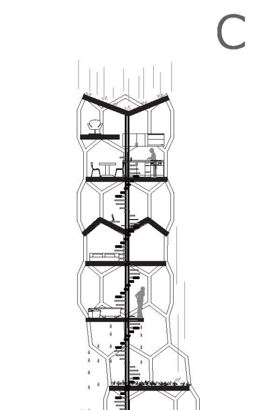
section;scale:1/200
