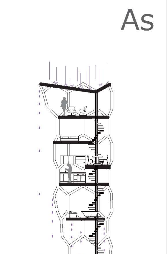
section;scale:1/200
