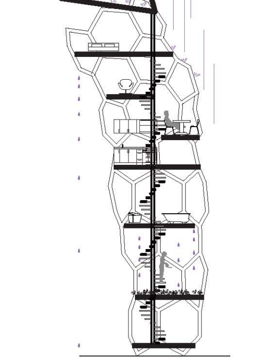
section;scale:1/200
