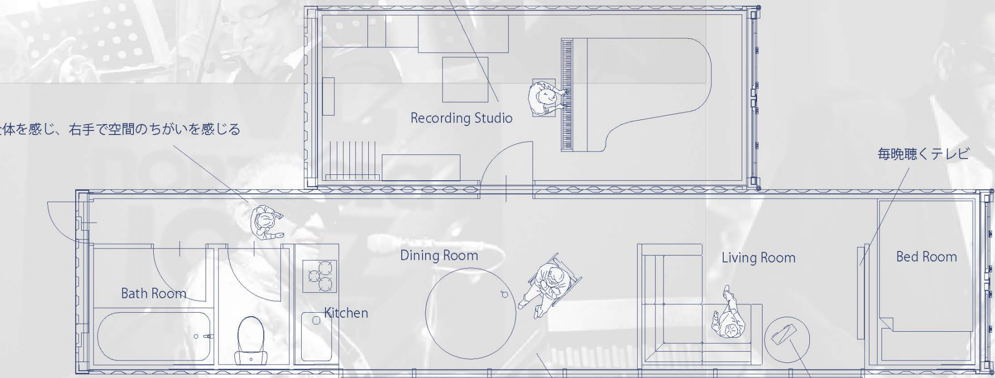
Floor Plan S=1:50
