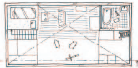
upper floor plan S=1/100
