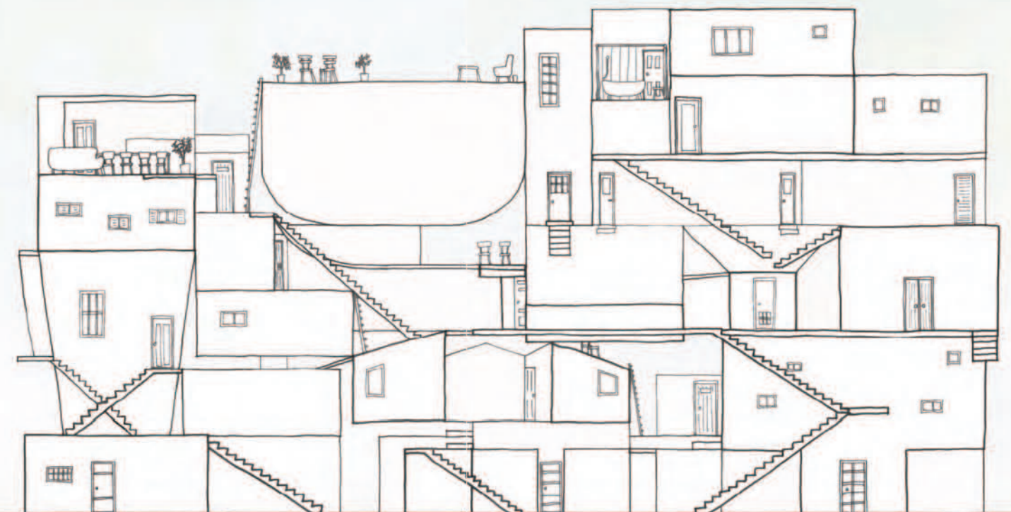
D-D section S=1/100
