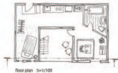
floor plan S=1/100
