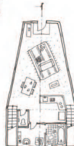
lower floor plan S=1/100
