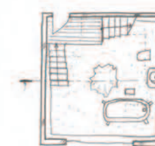
lower floor plan S=1/100
